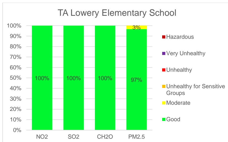
Figure 2: TALES AQI Distribution Summary — April through June 2021
