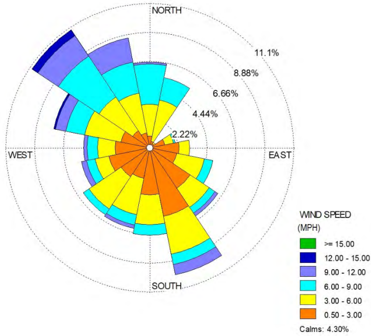
Figure 10: May 2021 Wind Rose
