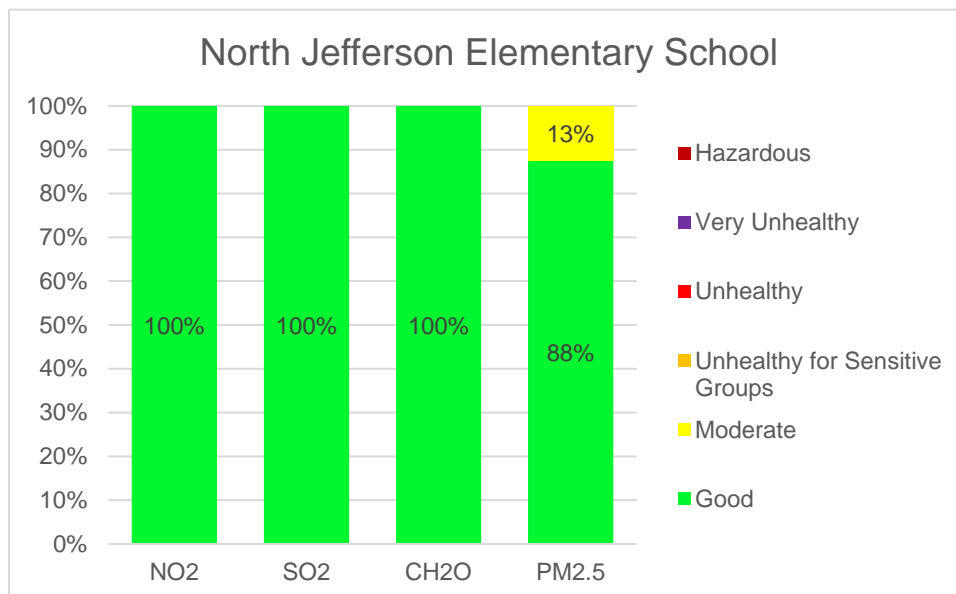
Figure 7: NJES AQI Distribution Summary — April through June 2021
