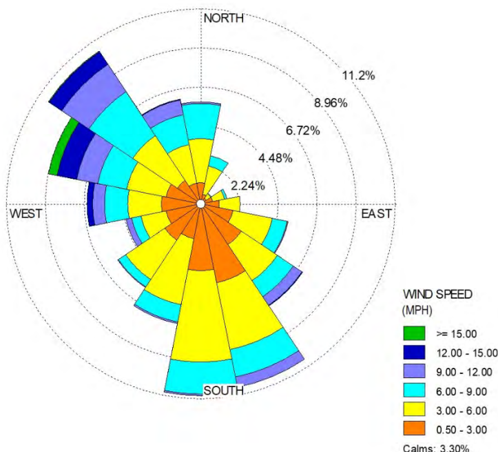
Figure 12: April through June 2021 Wind Rose
