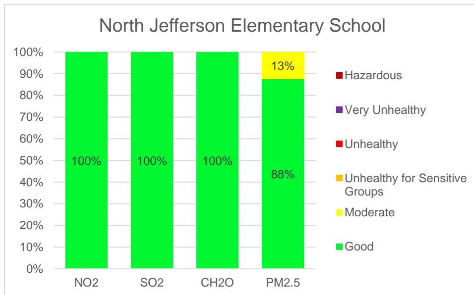
Figure 1: NJES AQI Distribution Summary — April through June 2021
