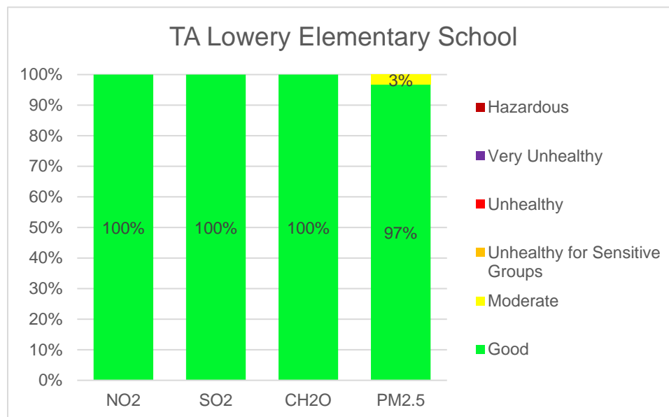
Figure 8: TALES AQI Distribution Summary — April through June 2021
