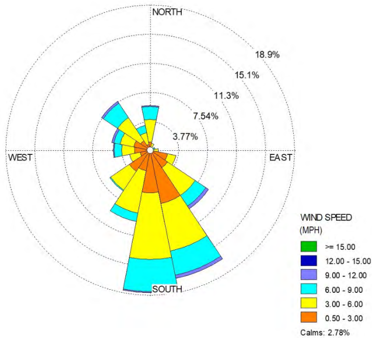
Figure 11: June 2021 Wind Rose
