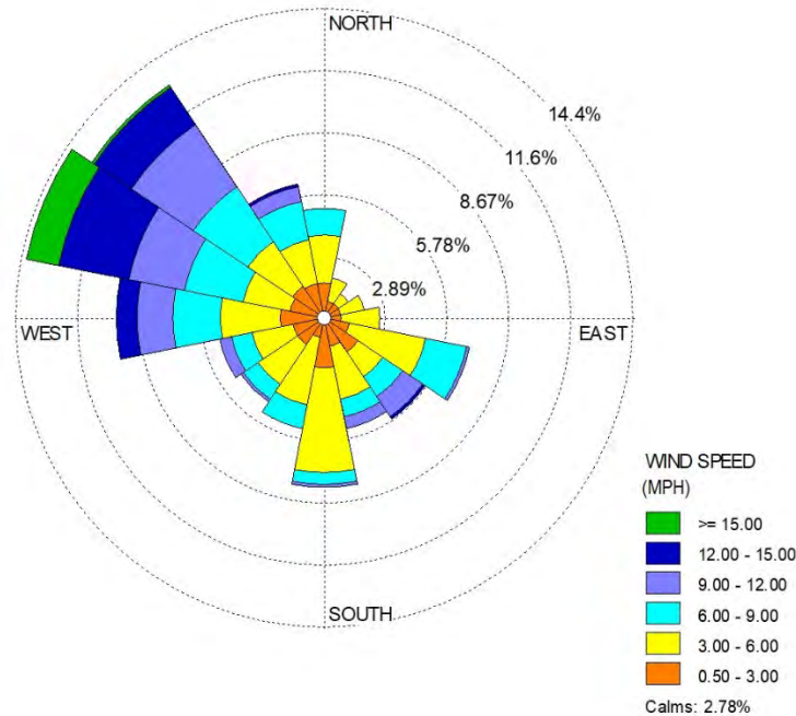
Figure 9: April 2021 Wind Rose
